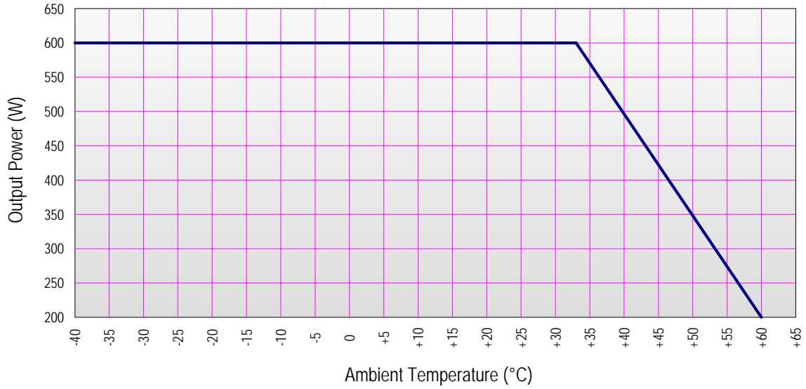
INMSW600-24/220 Power Derating Curve
