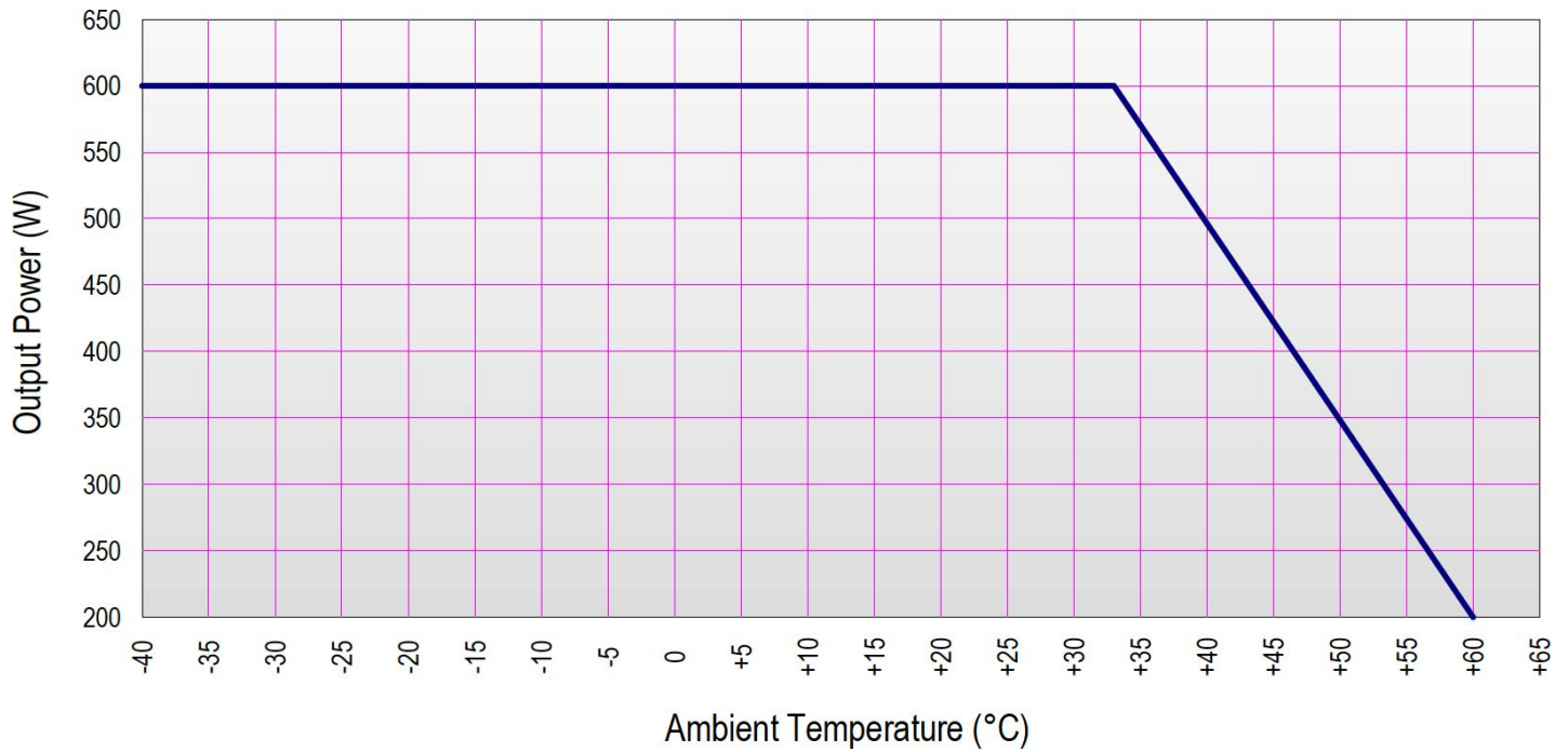
INMSW600B-24/220 Power Derating Curve
